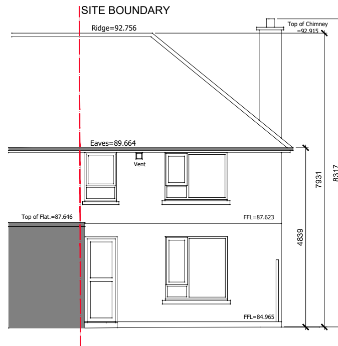
01 EXISTING SIDE ELEVATION (EAST) PL03 1 : 100
