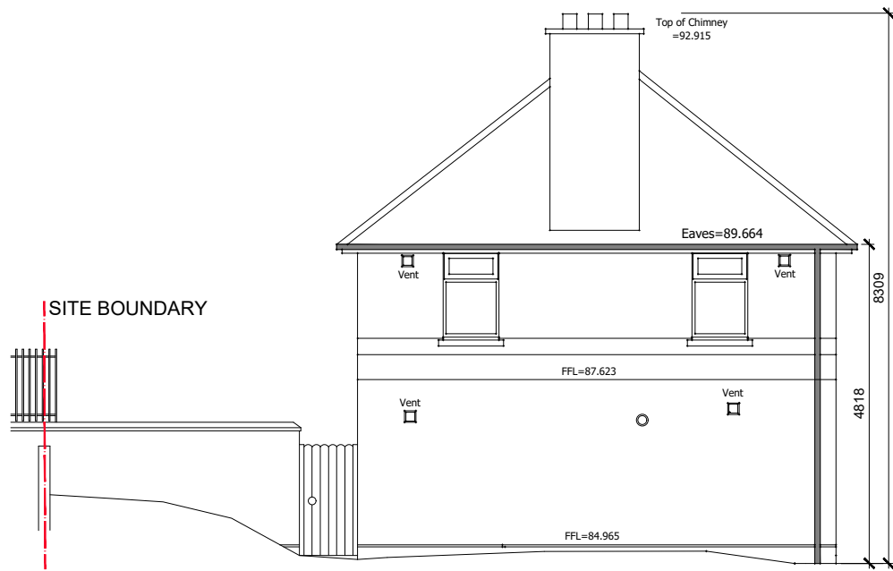
01 EXISTING SIDE ELEVATION (NORTH) PL03 1 : 100
