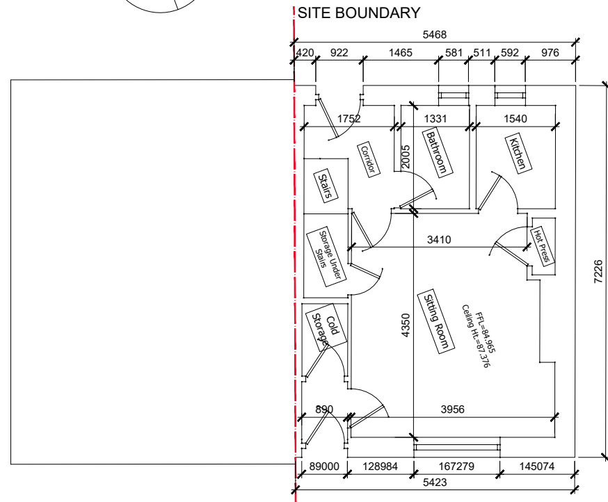
01 EXISTING GROUND FLOOR PLAN PL03 1 : 100
